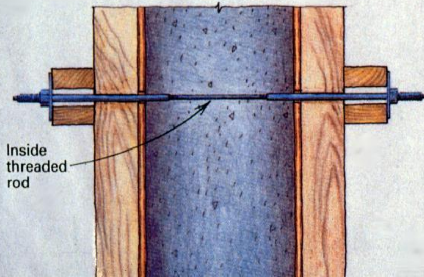
She bolts
