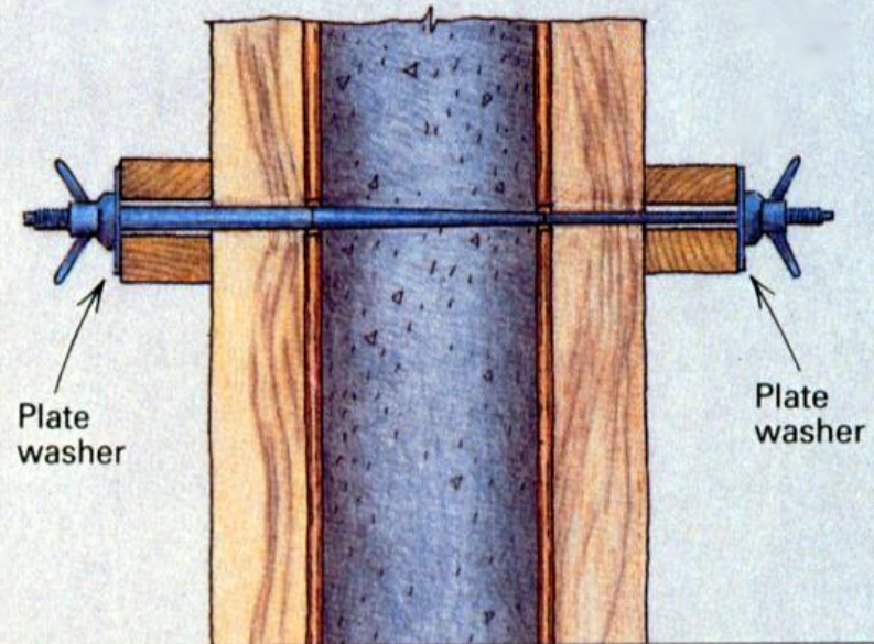
Taper tie
